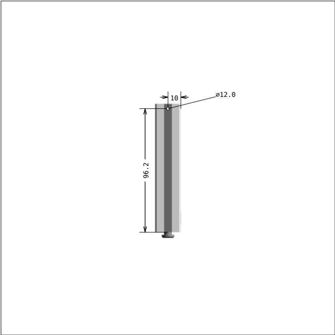
DRAWING 1, Pos 1 SIDE 1, bar length: 100.0 mm
